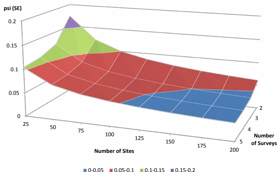
Figure 5: The relationship between the precision of occupancy estimates (the proportion of sites occupied by a species) varies depending on the number of sites surveyed and the number of repeat surveys undertaken at a site (e.g. the number of weeks cameras are deployed). When either the number of sites or number of surveys is increased the precision of the occupancy estimates improves. However, the improvement in the estimate is far better when the number of sites surveyed is increased. The colours on the graph represent the precision (SE = standard error) of the occupancy estimate (psi). Lower values mean the estimate is more precise.
